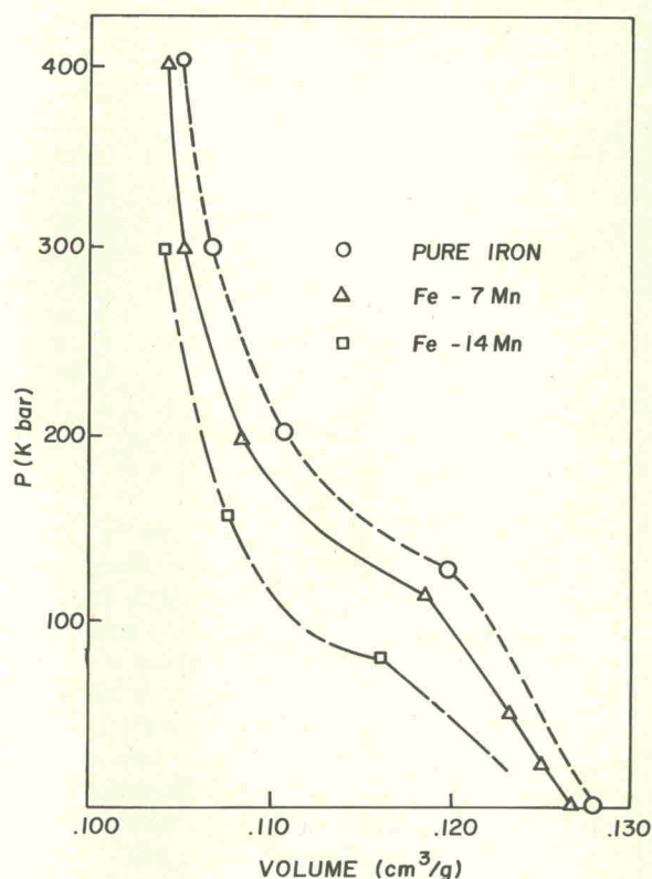
FIG. 11. Hugoniot curves for Fe-Mn alloys.
