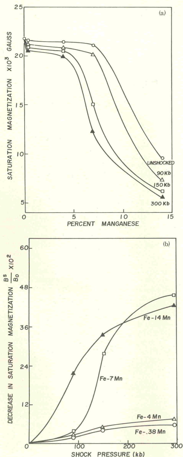
FIG. 10. (a) Saturation magnetization as a function of manganese content for shocked and unshocked alloys. (b) Fractional change in saturation magnetization as a function of peak pressure.
